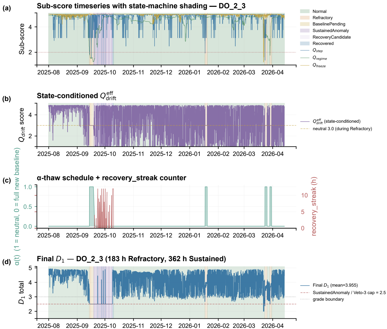
Figure V13. Causal six-state recovery machine — DO_2_3 case study
